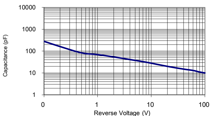
Figure 5: Typical Junction Capacitance
