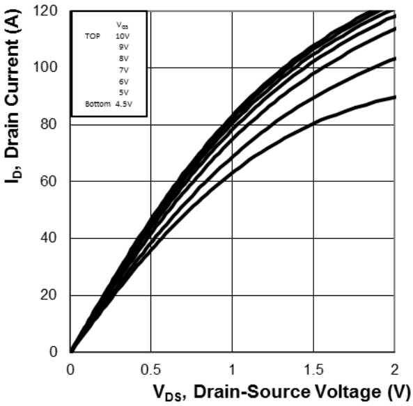
Figure 5: On-Region Characteristics
