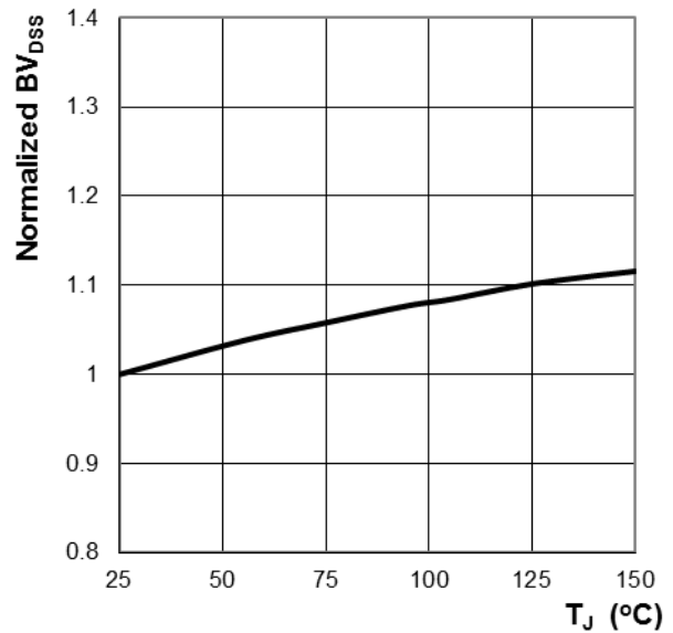
Figure 4: Normalized BV_{DSS} vs. T_J
