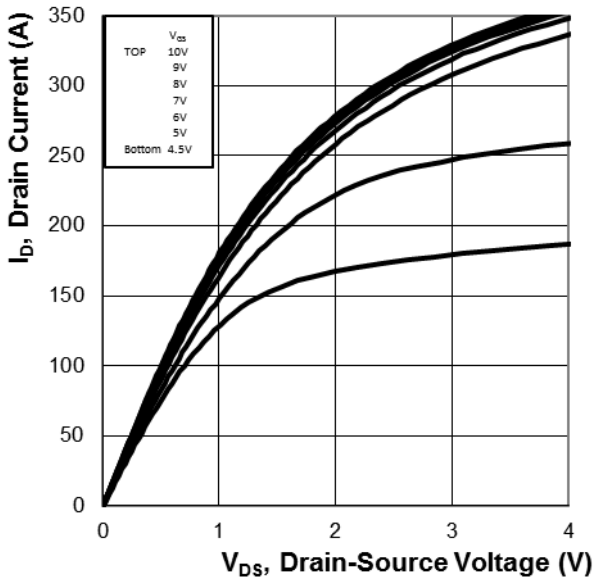
Figure 5: On-Region Characteristics
