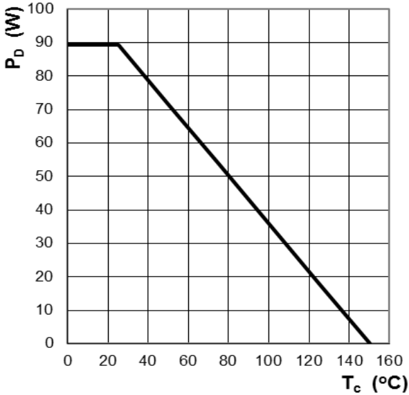
Figure 1: Power Dissipation
