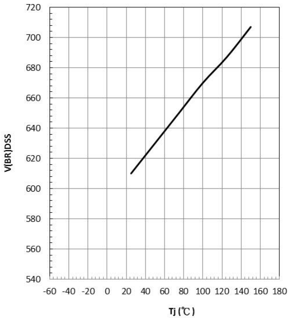
Fig 11: Drain-source breakdown voltage
