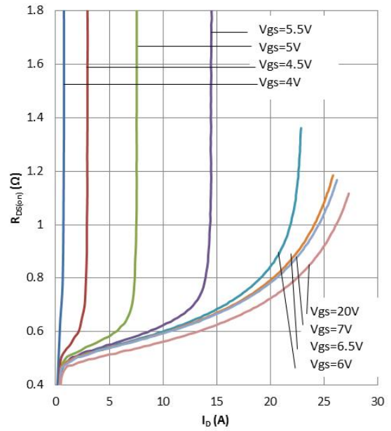
Fig 6: Typ. Drain Source On-Resistance
