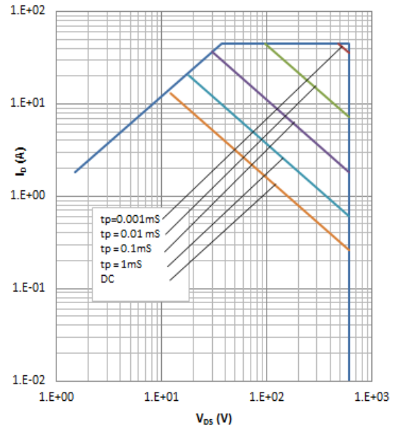
Fig 2: Safe operating area
