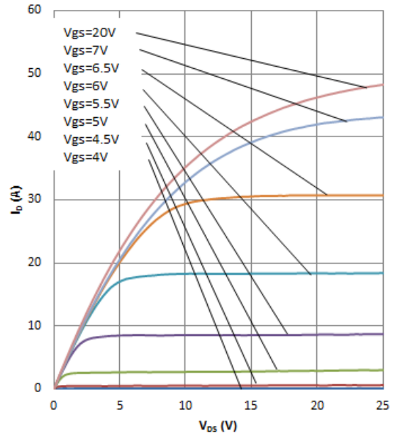
Fig 4: Typ. Output Characteristics
