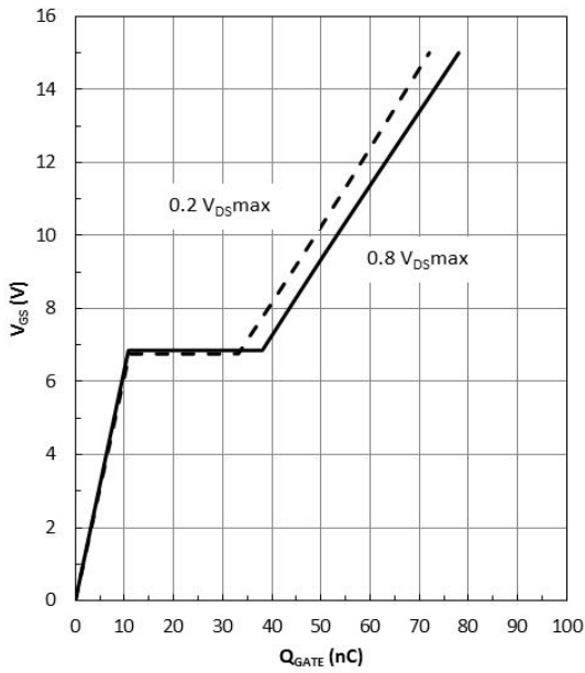
Fig 9: Typ. Gate Charge diode
