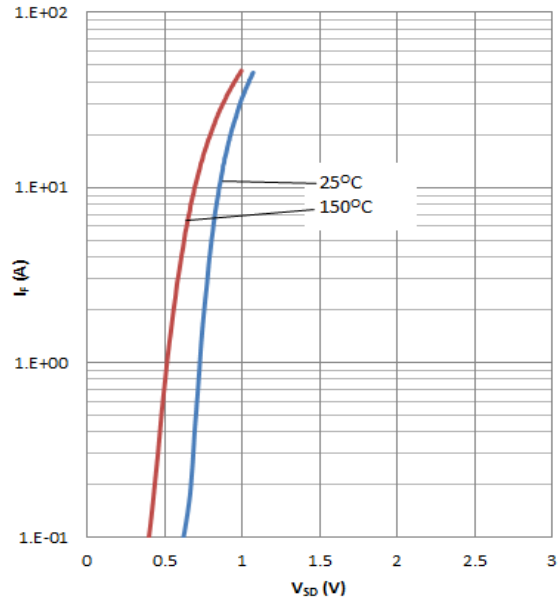
Fig 10: Forward characteristics of body diode
