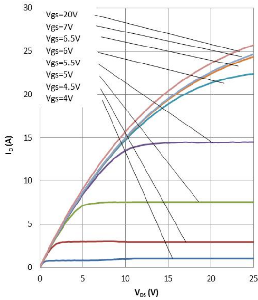
Fig 5: Typ. Output Characteristics
