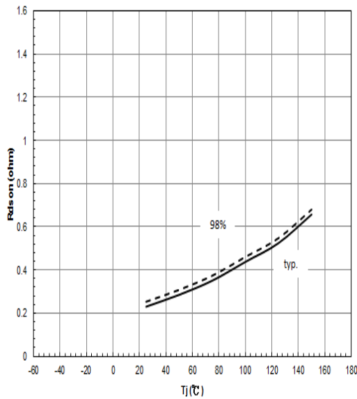
Fig 7: Drain-Source On-state Resistance
