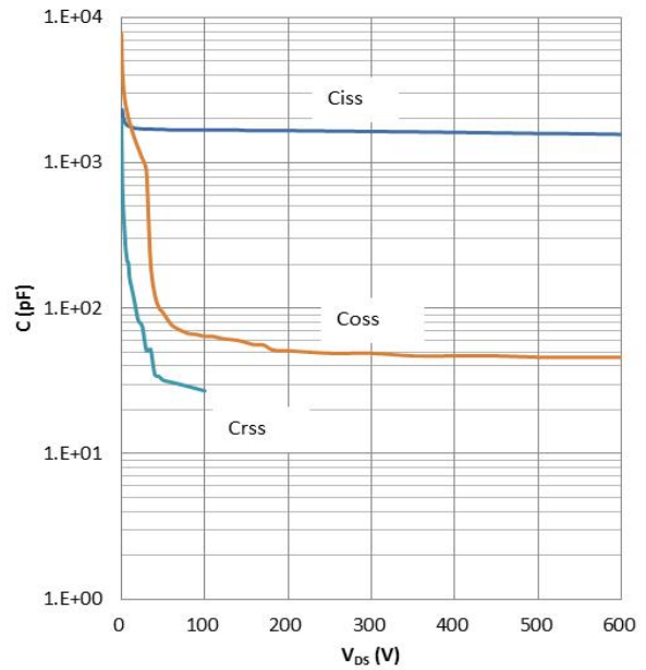
Fig 12: Typ. Capacitances energy
