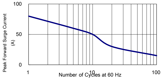
Figure 2: Maximum Repetitive Surge Current
