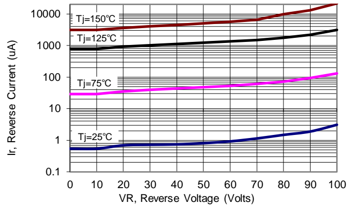
Figure 4: Typical Reverse Current
