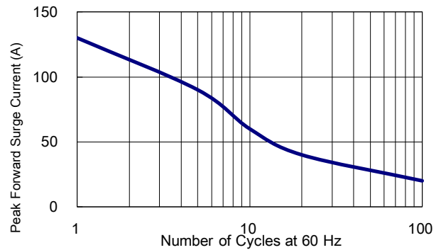
Figure 2: Maximum Repetitive Surge Current
