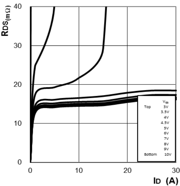
Figure 5: RDS(ON) vs. Drain Current and Gate Voltage
